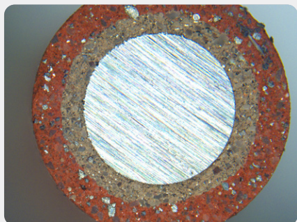
Basic coating outside, rutile cover inside
